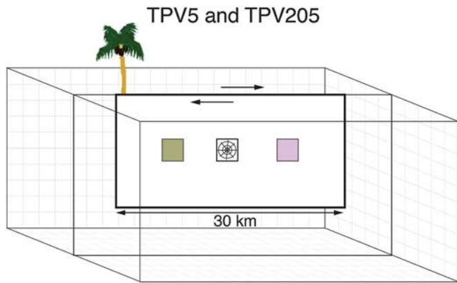
▲ Figure 4. TPV5: The earthquake rupture is artificially nucleated in a square zone at the center of the fault surface. The rupture then spontaneously propagates over the rest of the fault surface. As it propagates away from the nucleation zone, it encounters two square patches with initial stress conditions that are different from the rest of the fault surface. TPV205 is the same as TPV5; TPV205 is a convergence test with respect to grid size.
