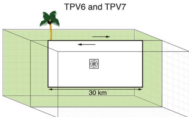
▲ Figure 5. TPV6 and TPV7: The earthquake rupture is artificially nucleated in a square zone at the center of the fault surface. The rupture then spontaneously propagates over the rest of the fault surface. The fault surface is the boundary between rocks with different elastic moduli. This material contrast is stronger for TPV6 than it is for TPV7.
