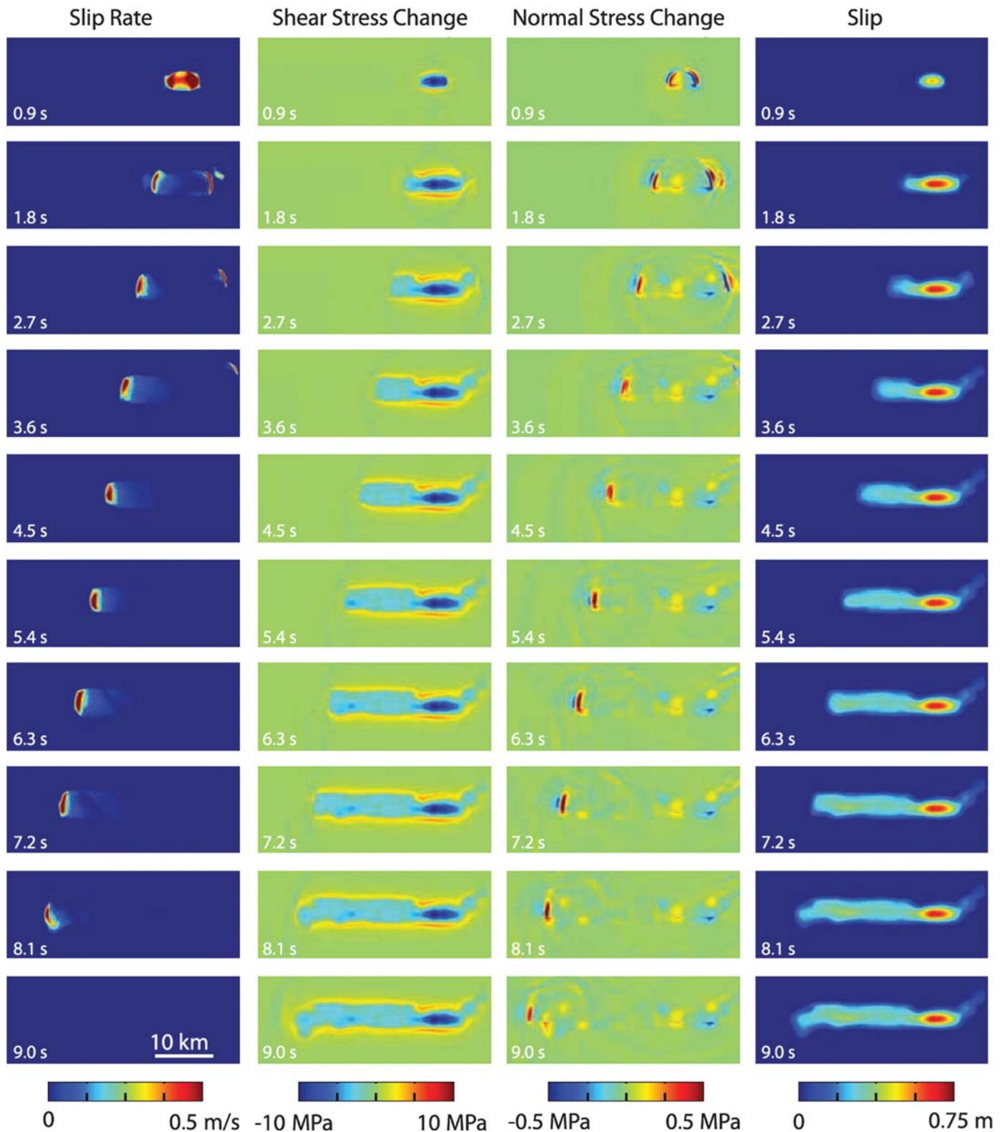
▲ Figure 2. Example of results produced using dynamic (spontaneous) earthquake rupture simulation code MAFE (Ma et al. , 2008). Time-dependent pattern of an earthquake rupture on a planar vertical strike-slip fault surface. The simulated earthquake, in this case the Ma et al. (2008)-favored model of the 2004 M 6.0 Parkfield, California, earthquake, was nucleated at 0.0 s on the fault surface, centered at a depth of 8.1 km. The subsequent dynamic, spontaneously propagating rupture is shown in figure 5 of Ma et al. (2008) (reproduced here) as a time-evolving pattern of slip rate, shear stress change, normal stress change, and slip on the fault surface, in snapshots starting at 0.9 s after nucleation.
