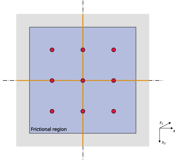
Figure 2: Observation points, lines, and region for model outputs. Local time series is output at select points (red circles). Slip, pore pressure, Darcy velocity and stress evolution are output along two cross-section lines (orange lines). The region outlined in black illustrates the frictional region from which the source parameter time series is calculated.
